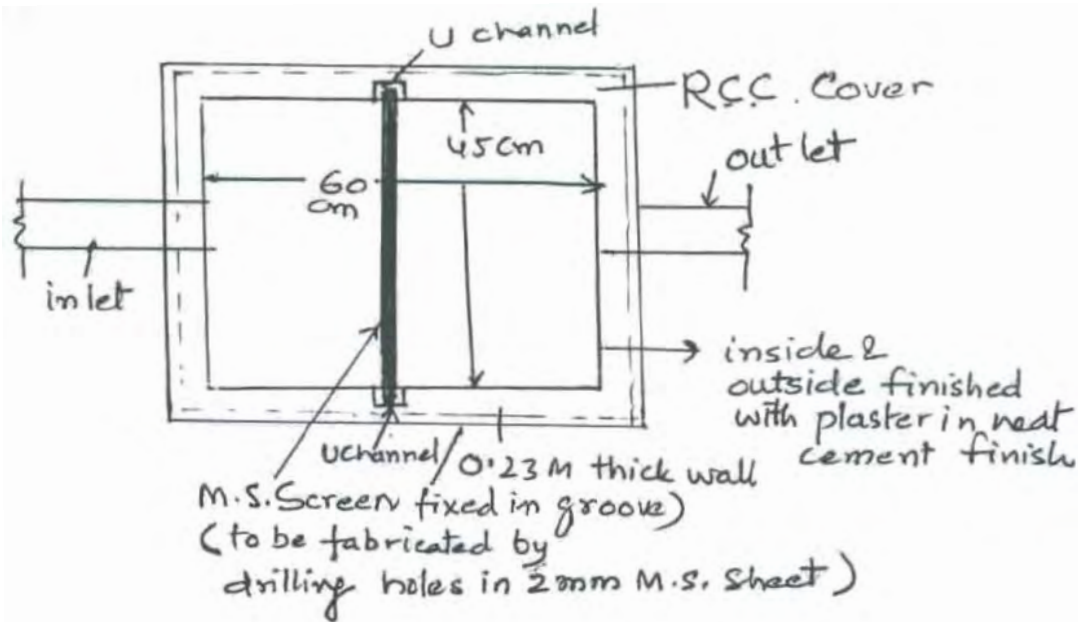
Chamber for screening of flow
