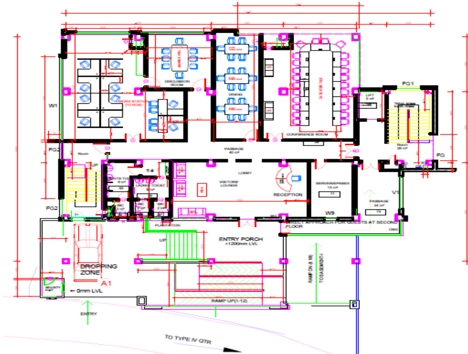
GROUND FLOOR
